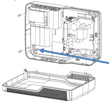
Fig. 1: Wall mounting
